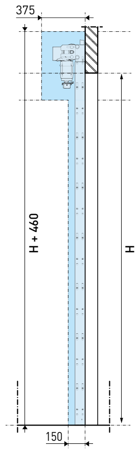
[ Dwarsdoorsnede ]
