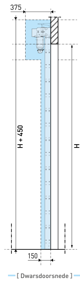
[ Dwarsdoorsnede ]
