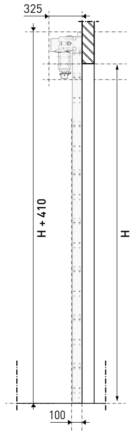
[ Dwarsdoorsnede ]
